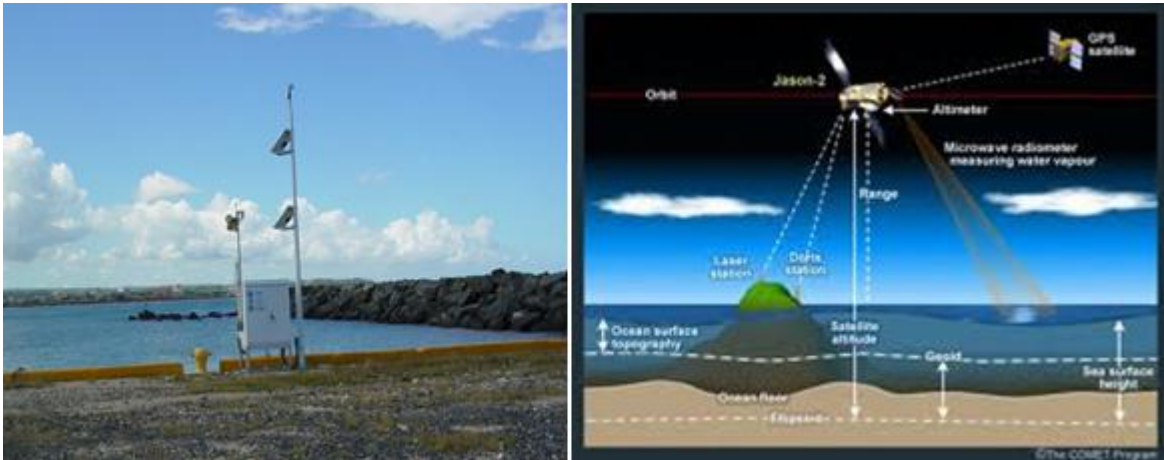
Figure 20. Methods for measuring sea level: tide gauge (relative) and satellite (absolute)
